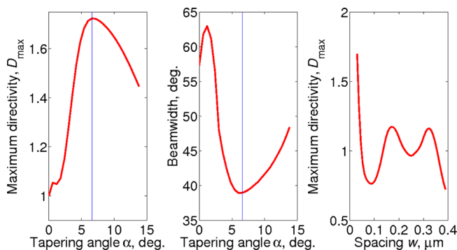
FIG. 3. (Color online) (a) Maximum emission directivity D_{max} and (b) beamwidth of the tapered 42-element Yagi-Uda nanoantenna as a function of \alpha . The straight lines highlight \alpha_{opt} = 6.6^\circ . (c) D_{max} at \alpha_{opt} = 6.6^\circ as a function of the spacing w .
